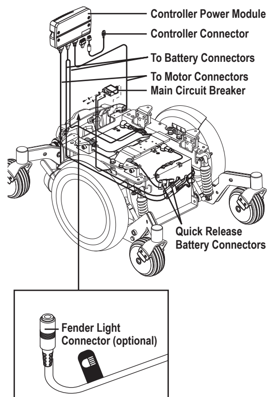
Figure 1. Electrical Components
