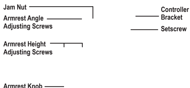
Figure 16. Seatback/Armrest Adjustment
