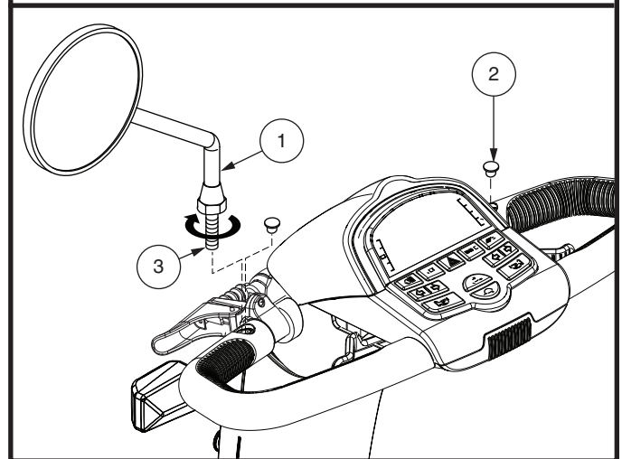
Figure 18. Mirror Installation and Positioning
