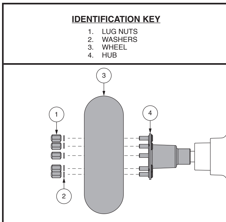
Figure 26. Wheel Removal
